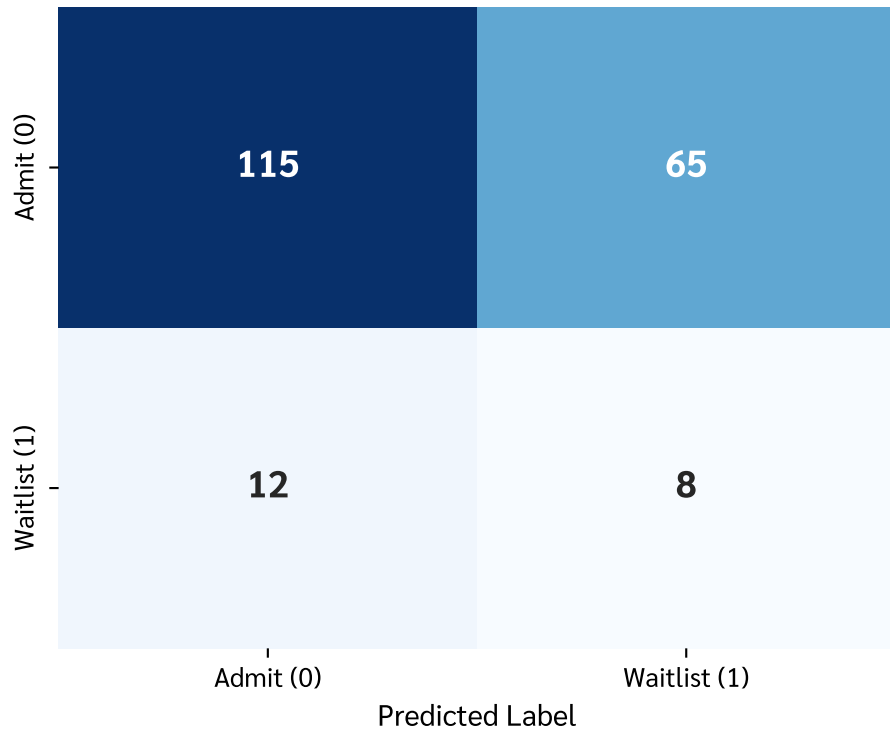
Decision Tree Confusion Matrix
