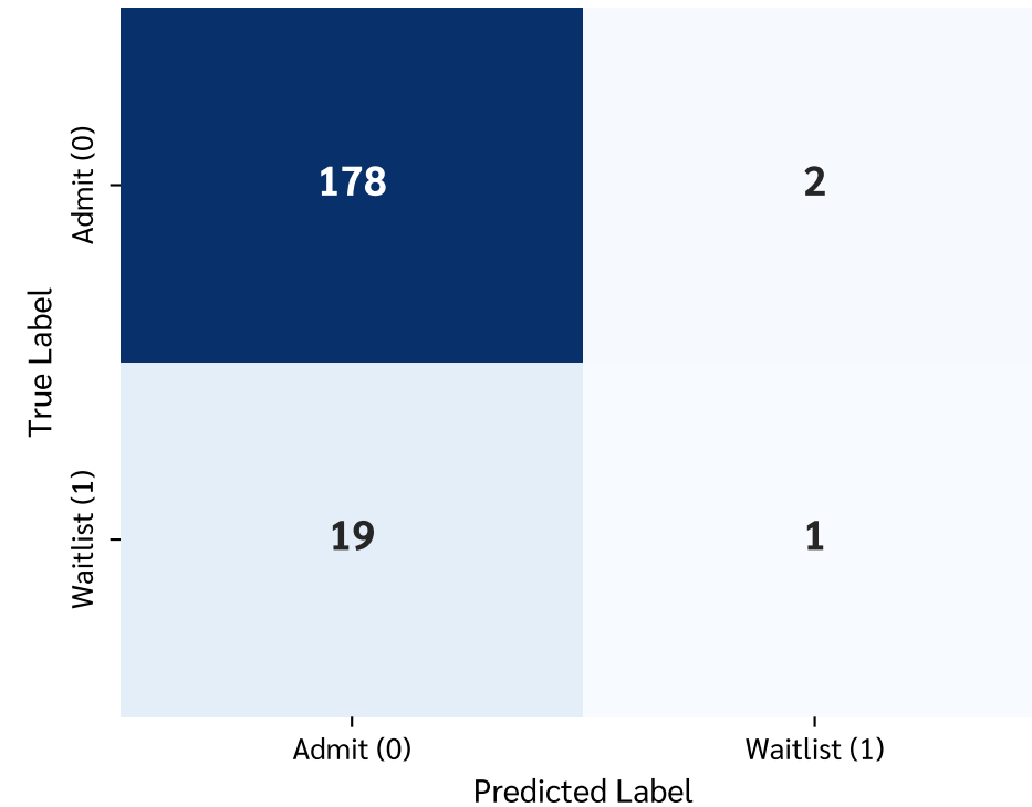
Gradient Boosting Confusion Matrix
